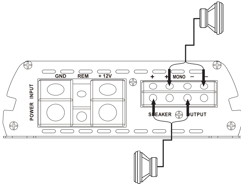
VL4000D FRONT PANNEL
